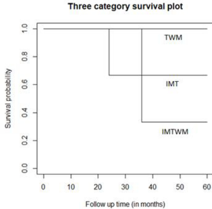
Figure 3: Overall survival analysis of the three groups i.e immature teratoma(imt), teratoma with bmalig-nancies(twm), immature teratoma with malignancies(imtwm)
